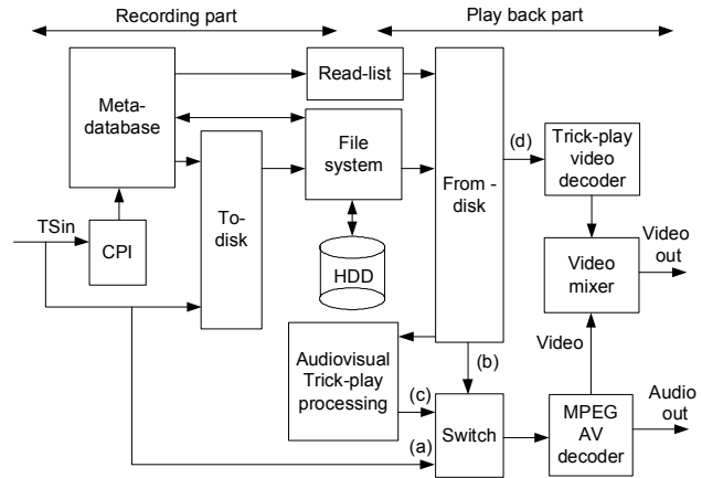
Fig. 2. HDD-based PVR architecture. Switch in position (a) indicates the real-time viewing mode; in case (b), the play-back of delay viewing; and in case (c), the trick-play operation mode for the normal play trick-play fragments, the fast search trick-play is flow in indicated by (d).
