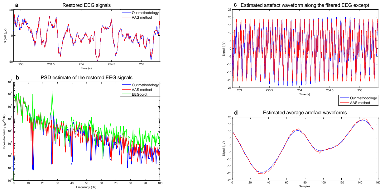
FIG. 4 COMPARISON BETWEEN THE RESULTS OBTAINED BY OUR METHODOLOGY AND THE AAS METHOD: (A) RESTORED EEG SIGNALS (B) PSD ESTIMATE OF THE RESTORED SIGNALS; (C) ARTEFACT WAVEFORMS FOR THE ENTIRE EEG EXCERPT; (D) AVERAGE ARTEFACT WAVEFORMS (155 SAMPLES)
