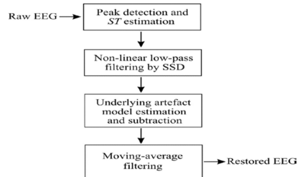
FIG. 1 PROPOSED ALGORITHM STRUCTURE FOR GRADIENT ARTEFACT MODELLING AND EEG RESTORATION
