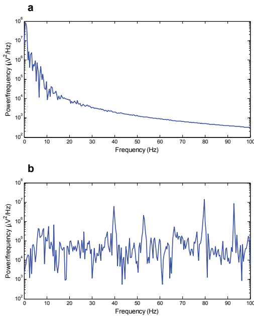
Figure 3: (a) Power spectrum of the fitted spline curve shown in figure 2b; (b) power spectrum of the subtraction of such a spline from the raw EEG of figure 2a. The gradient artefact frequencies are contained in (b).
