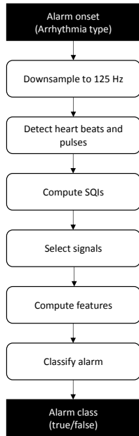
Figure 1. Flowchart of the algorithm
